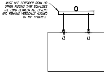
EXTERIOR WALL PANEL
