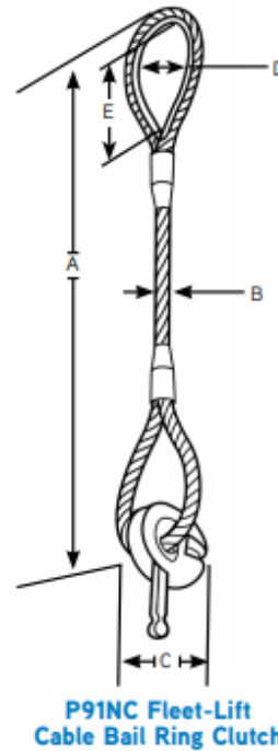
P91NC Cable Bail Ring Clutch
