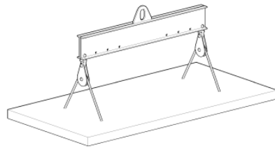
* RECOMMENDED EQUALIZED LIFT RIGGING METHOD PIECE 5, 6
