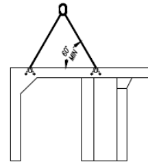
* SINGLE PERIMETER MODULE
