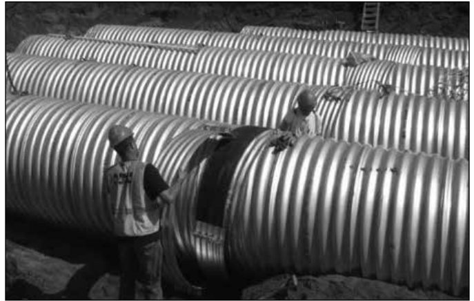
Installation of corrugated band with flat neoprene gasket
