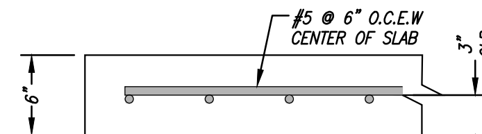
POURED IN PLACE BASE SLAB DETAIL
